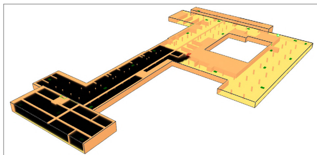
Smoke spread after 30 minutes.
