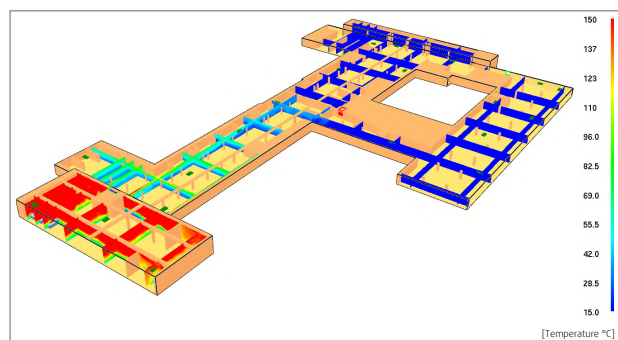
Spread of temperature within 30 minutes.
